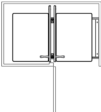
Final appearance of the swing-out tray for right opening
